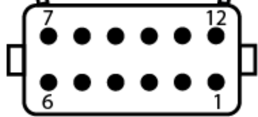
12 Pin - Female Back View
